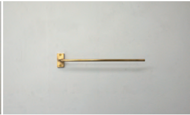
sen-60 タオルハンガー 大 4,800yen+tax size / W350 D50 material / brass accessories / M4 brass countersunk screw
