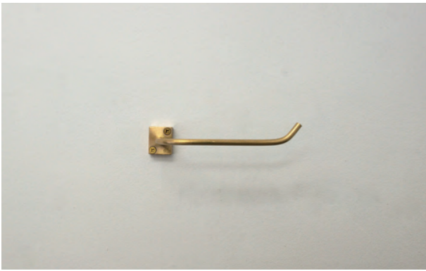
sen-62 ペーパーホルダー 4,800yen+tax size / W125 D75 material / brass accessories / M4 brass countersunk screw
